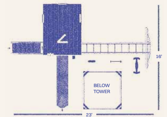
OVERHEAD VIEW
